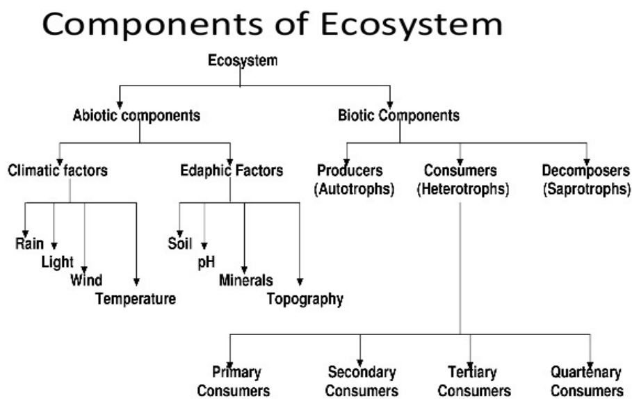
Figure 1.1: Components of the Ecosystem
